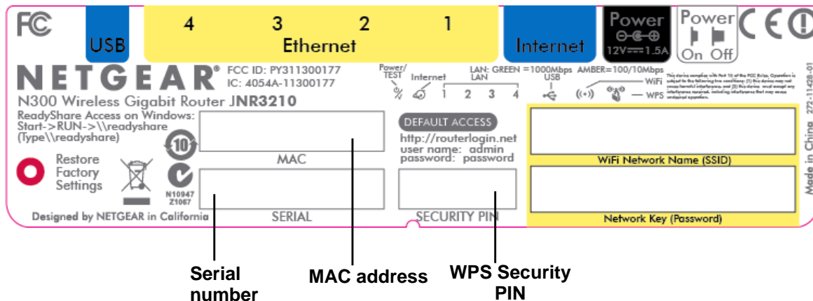
Figure 1. Label on router bottom
