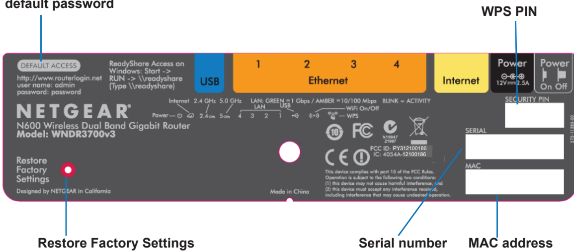
Figure 3. Label on router bottom
