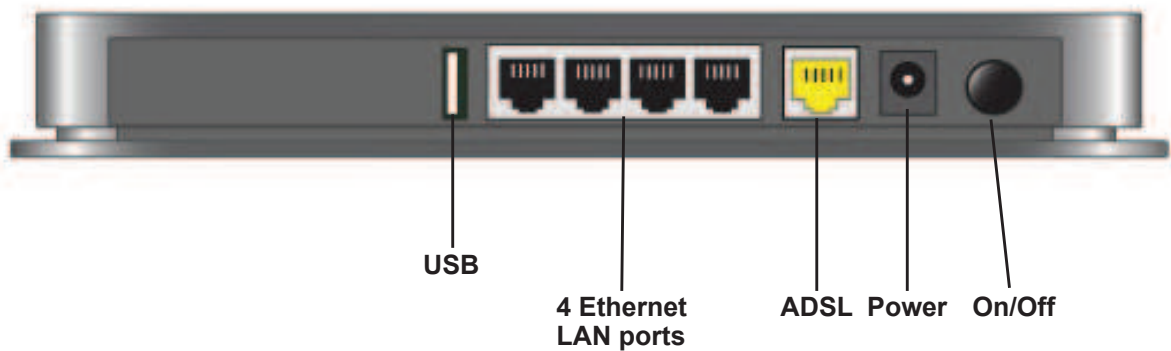
Figure 2. Back panel
