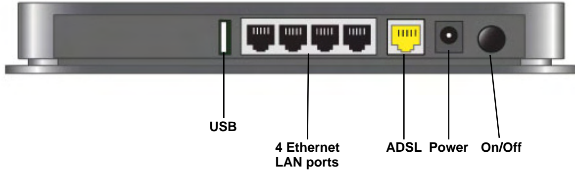
Figure 2. Back panel
