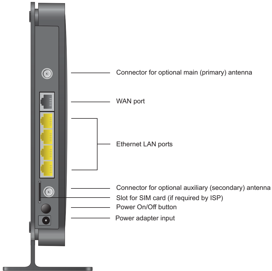
Figure 3. Router, rear view
