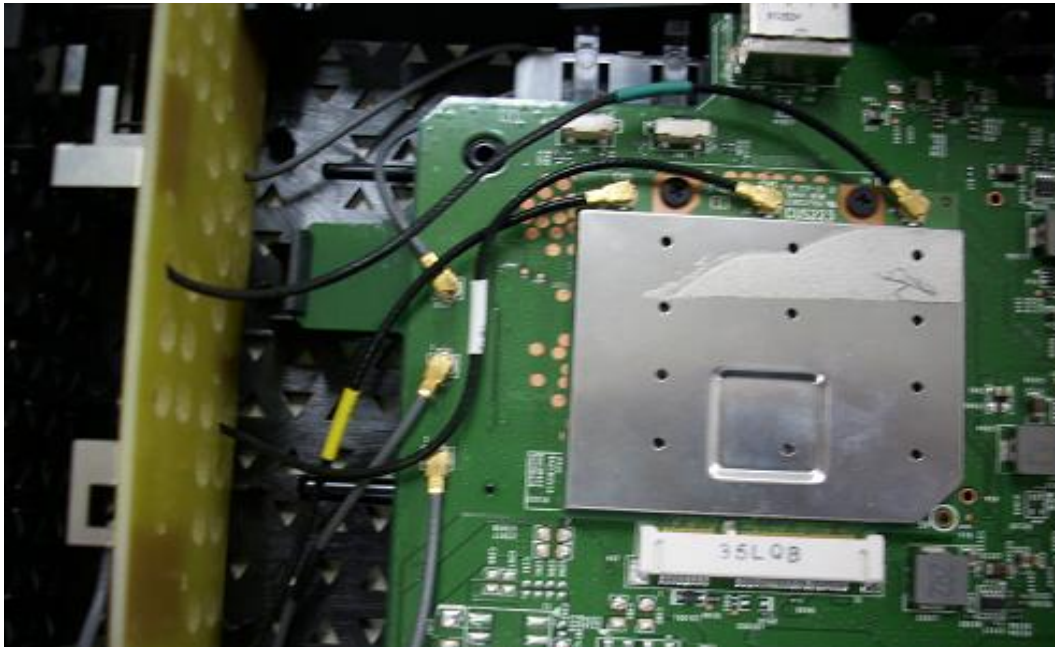
Step-4: Connect three external Wi-Fi antennas on I-PEX connectors.
