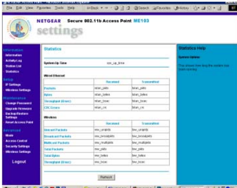
Figure 17: Statistics Screen
