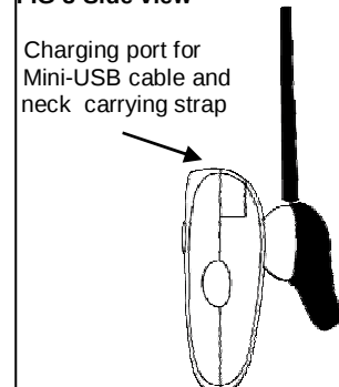
FIG 3-Side view
