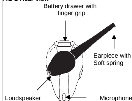
FIG 2-Rear view
