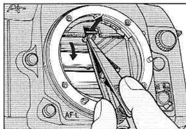
2. Slip the tip of the special tweezers (provided with optional screens) under the focusing screen release latch and pull outward to spring open the holder.
