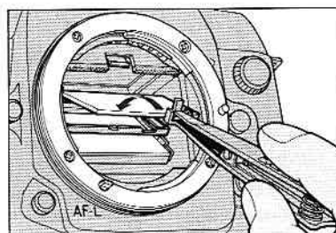
4. Carefully position the replacement screen in place, making sure the flash side is facing down.
