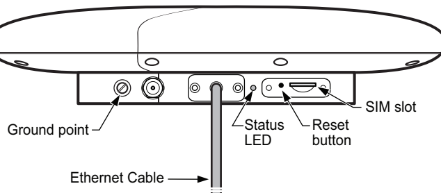
Figure 11 Location of physical interfaces on the Compact mono-band and ABA models of the Nokia FastMile 4G Receiver
