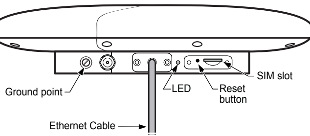
Figure 8 Location of physical interfaces on the Nokia FastMile Outdoor Unit
