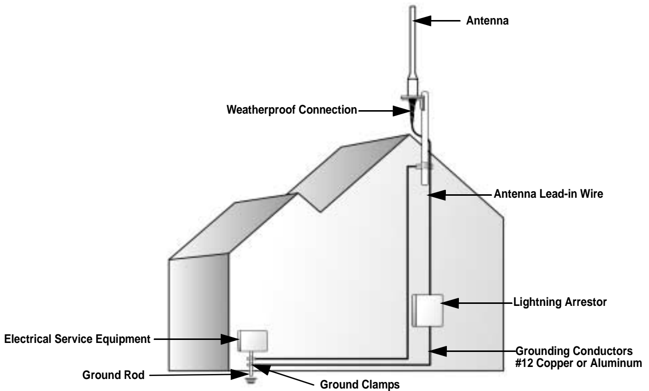
Grounding diagram
