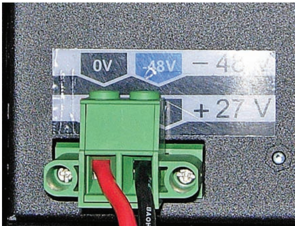
Figure 3-7 Cabling Power to +27 V dc BCUII
