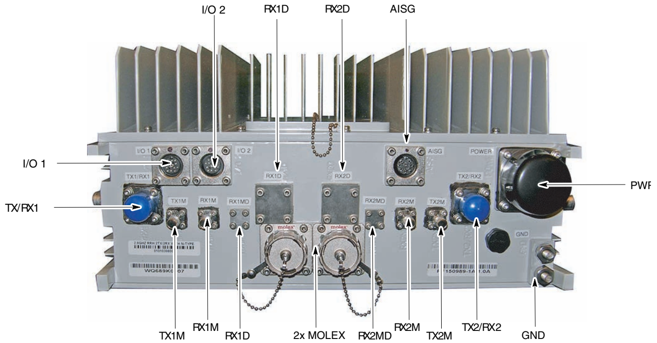
Figure 5-4 2.1 GHz RRH
