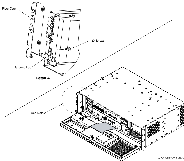
Figure 4-3 BCUII Grounding
