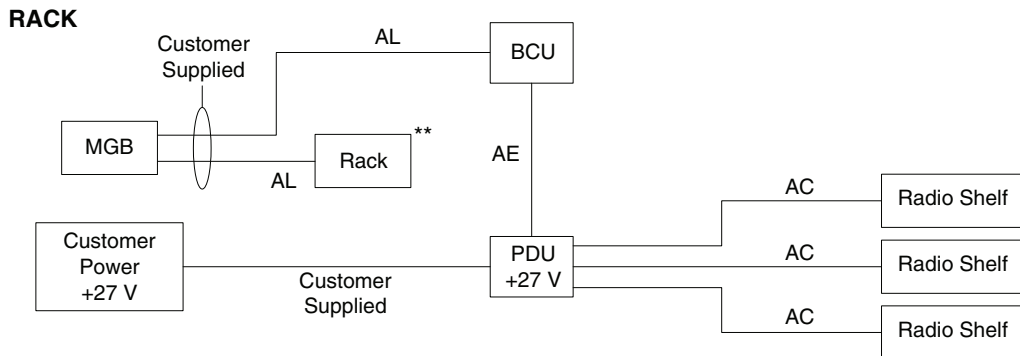
Figure 6-1 System Power Cabling
