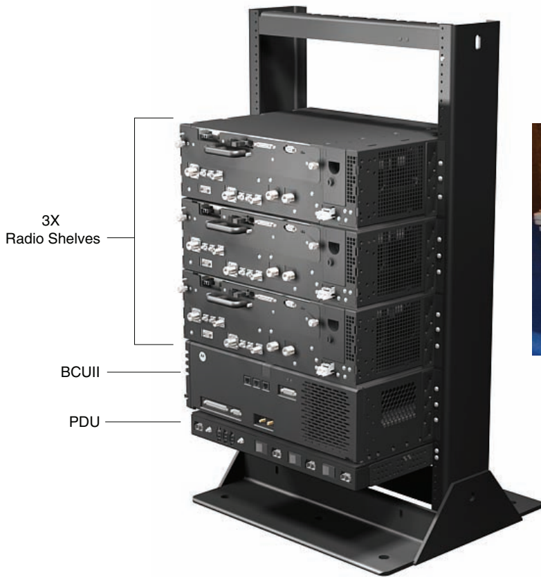
Figure 1-1 Major components
