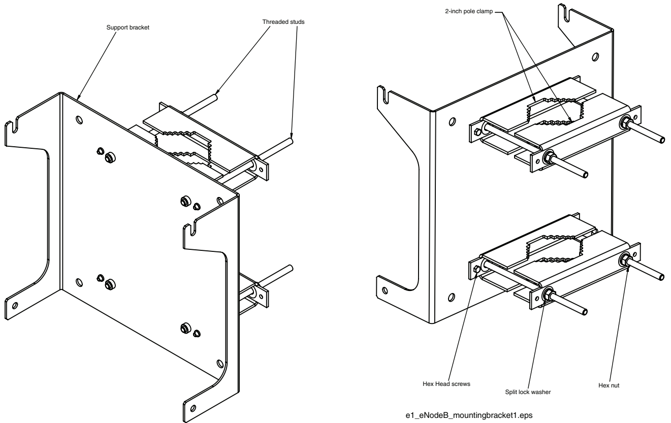
Figure 5-3 LTE 2.1/2.6 GHz RRH Mounting Bracket
