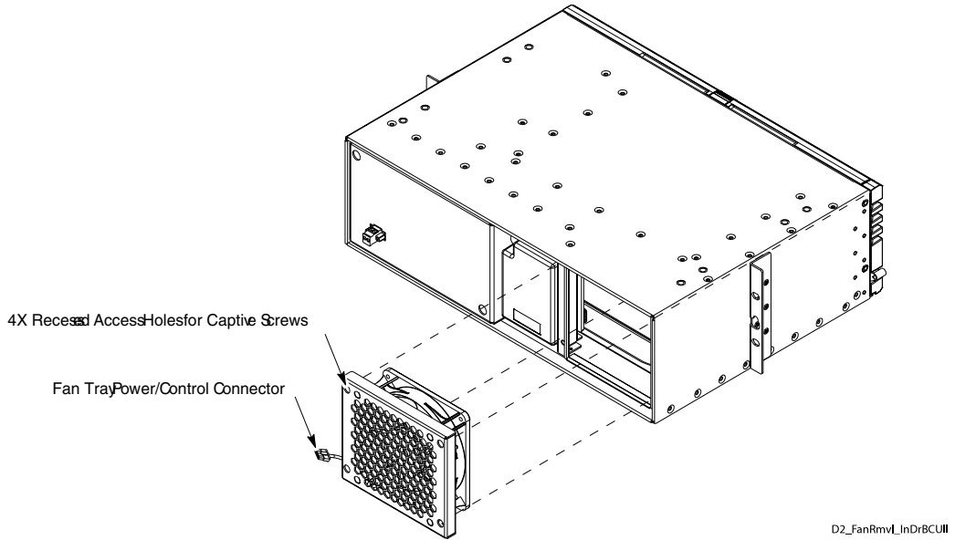
Figure 8-5 Fan tray removal and installation
