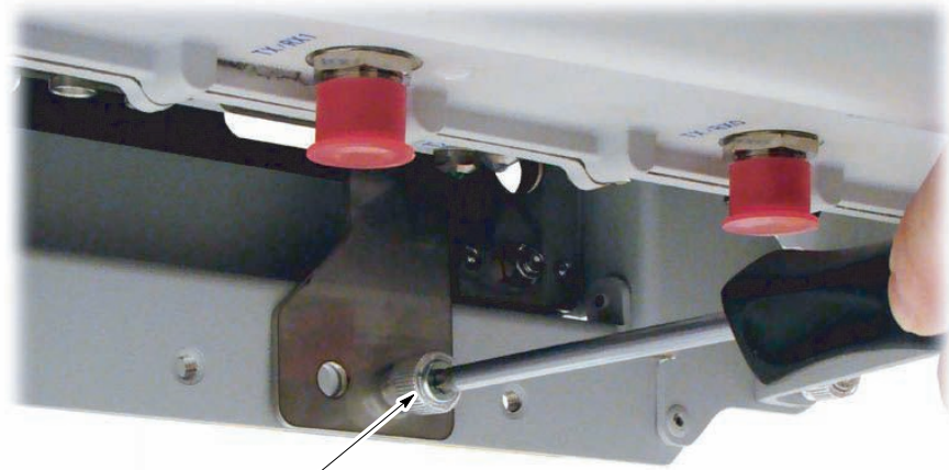
Captive M6 fastener
