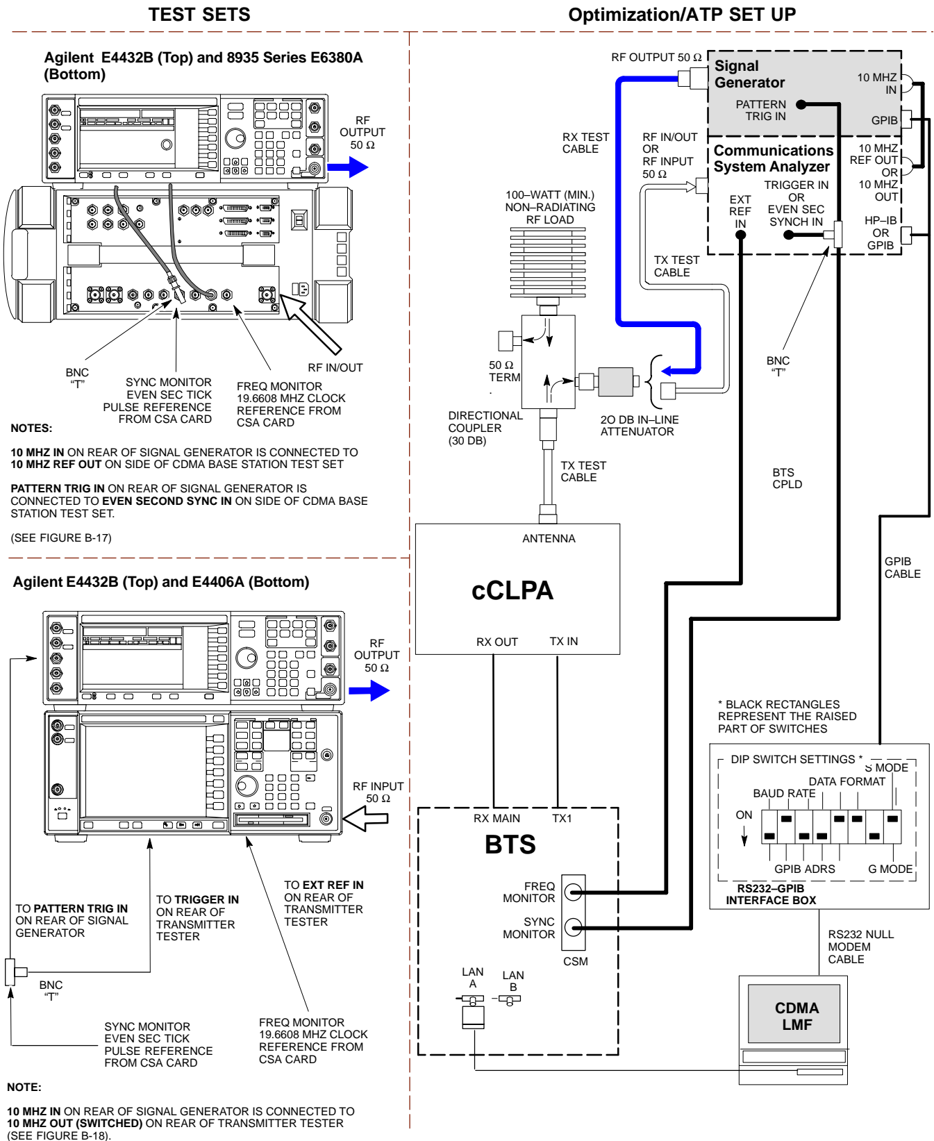
Figure 6-19: IS-95A/B and CDMA2000 1X ATP Test Setup Agilent Test Equipment
