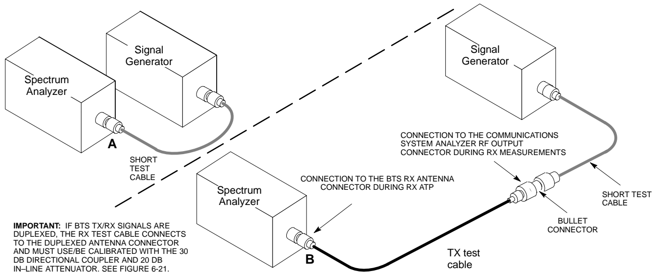
Figure 6-22: Cal Setup for Non-Duplexed RX Test Cabling Using Signal Generator & Spectrum Analyzer
