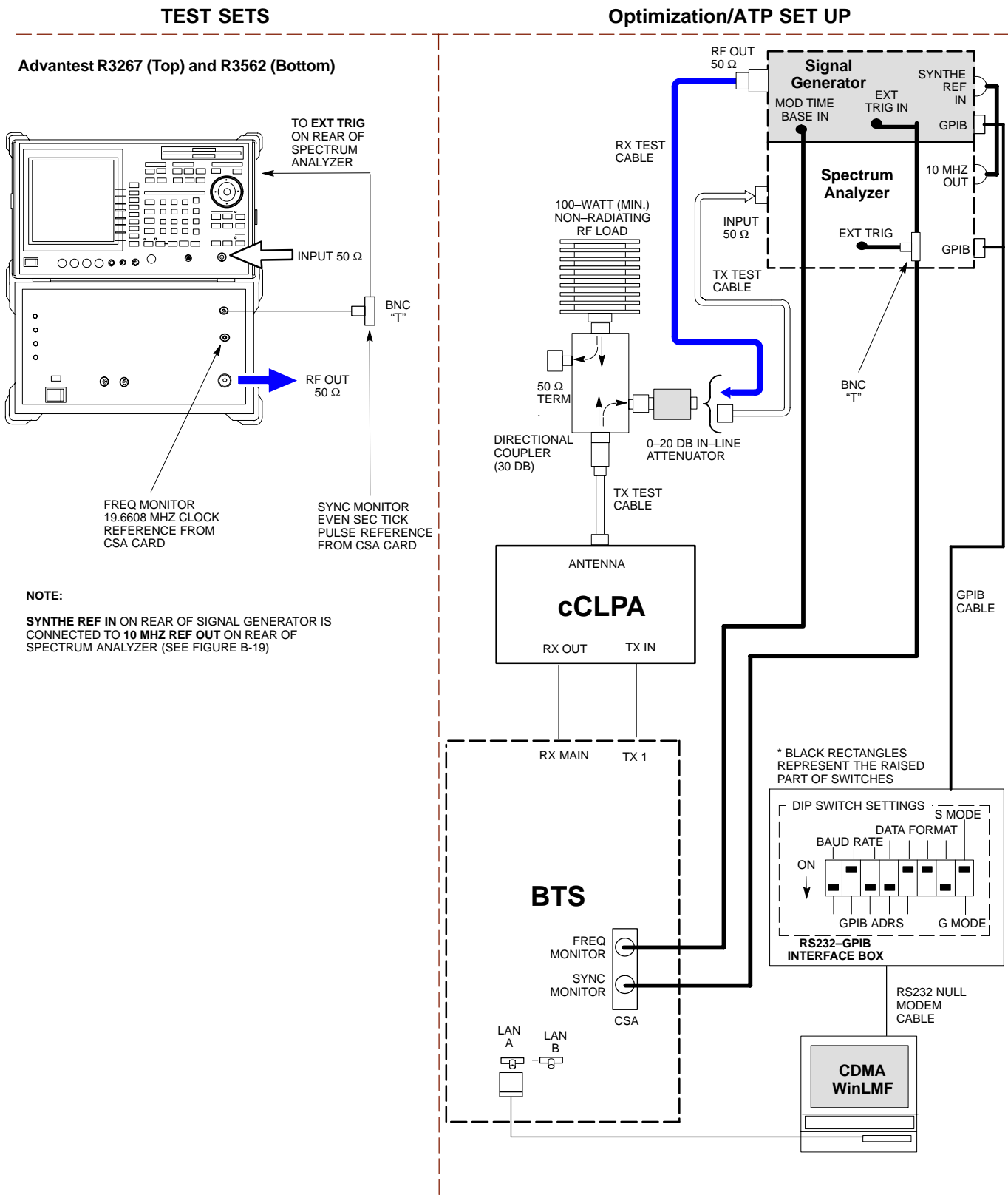
Figure 6-20: IS-95A/B and CDMA2000 1X Optimization/ATP Test Setup – Agilent E4432B/8935 Series E6380A and E4432B/E4406A Test Equipment
