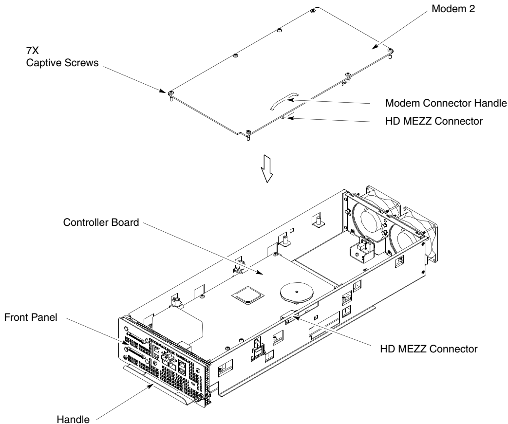
Figure 8-2 Removing and installing Modem 2
