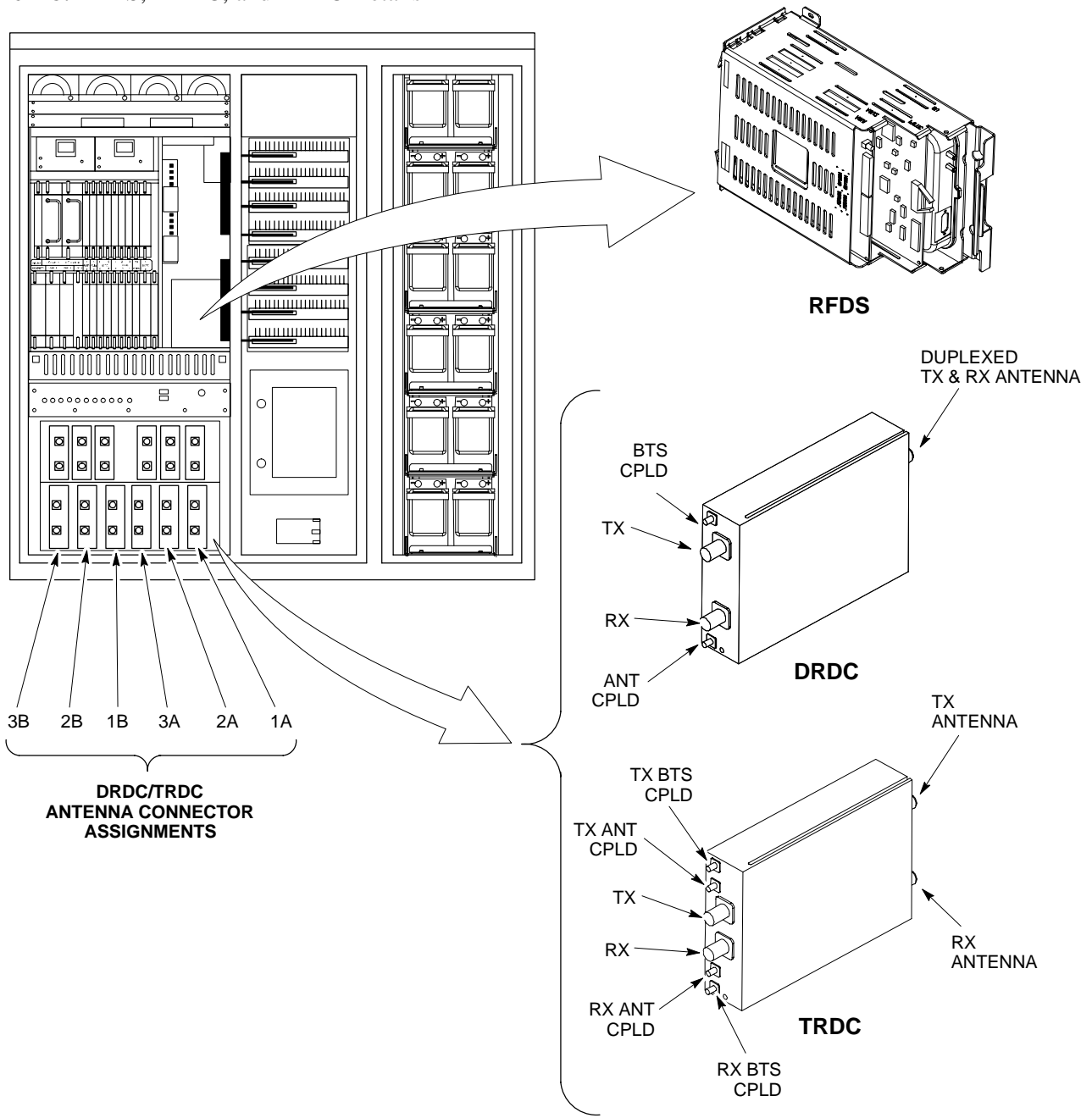
Figure 1-8: RFDS, DRDC, and TRDC Details
