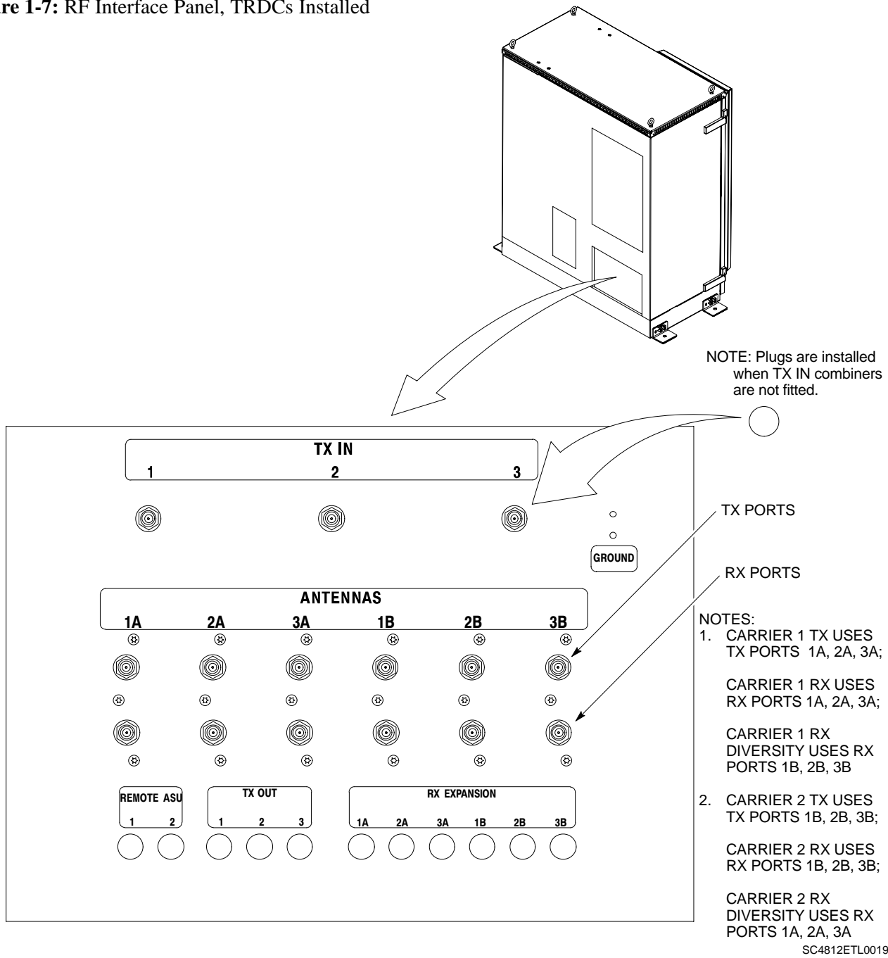
Figure 1-7: RF Interface Panel, TRDCs Installed
