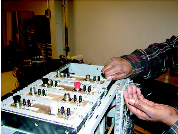
Figure 3-4 Installing the second set of IDRFs
