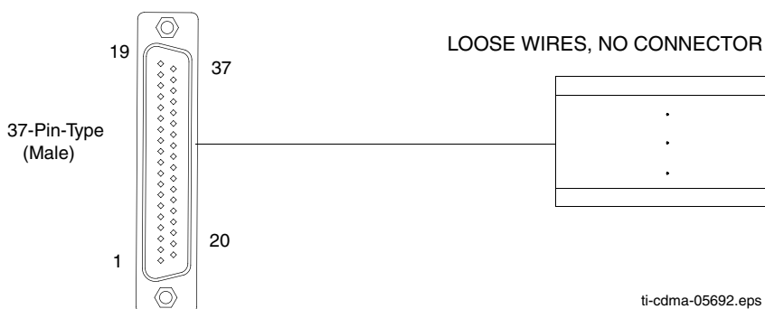
Figure 2-20 T1/E1 balanced span line cable (W) pin numbering
