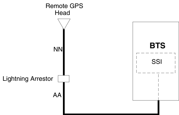
Figure 2-6 RGPS cabling diagram 3086039H14 RGPS cable, 304 m (1000 ft); part of Option 1472AL
