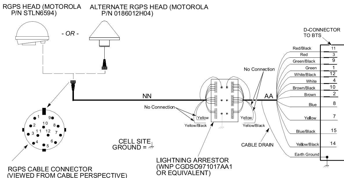
Figure 2-7 RGPS wiring
