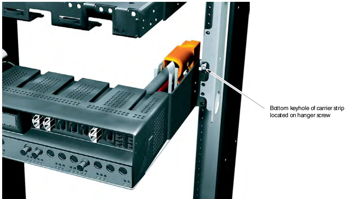
Figure 2-18 Carrier strip assembly keyhole screw locations
