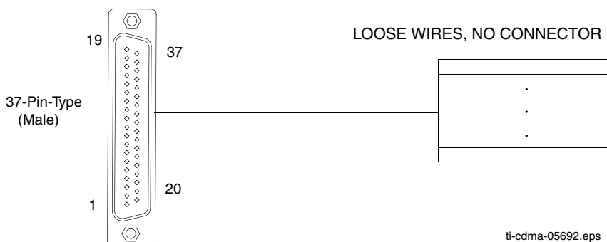
Figure 2-21 Customer alarm cable (X) pin numbering
