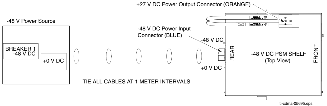
Figure 2-24 48 V DC power input cable (CC) wire tie-wrap example
