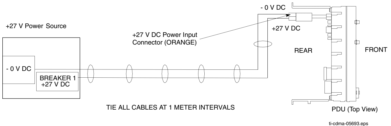
Figure 2-22 +27 V DC power input cable (DC) wire tie-wrap example
