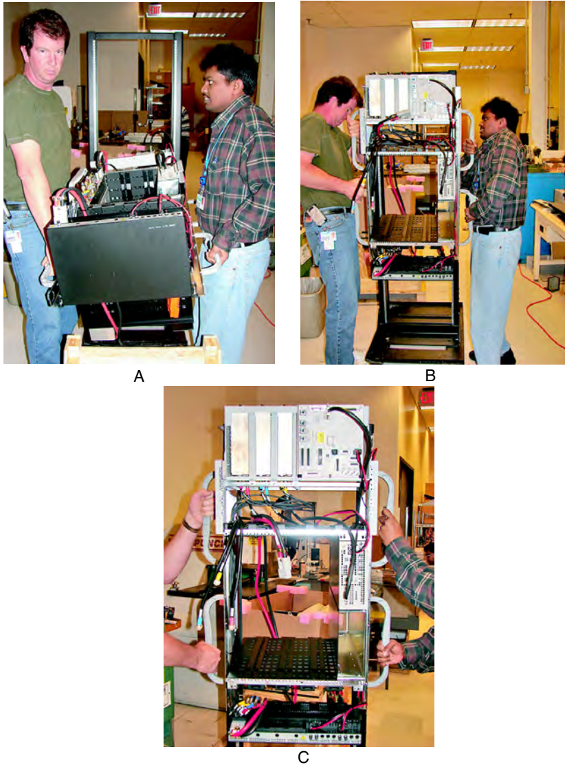
Figure 2-17 Lifting and hanging the carrier strip assembly on the rack (XMI shown removed)
