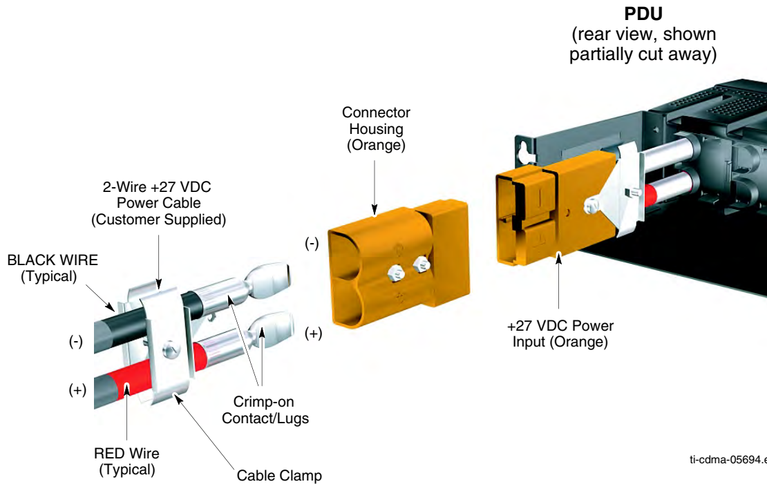
Figure 2-23 +27 V DC power input cable (DC) connector and connection to PDU
