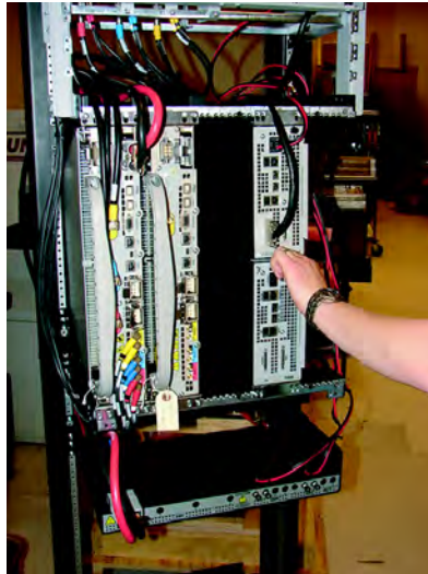
Figure 3-3 Installing a 2nd DMI
