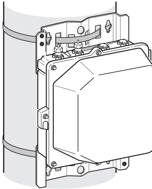
Figure 50 Securing the Enclosure To the Pole
