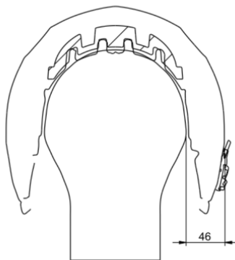
POSITION OF BLUETOOTH ANTENNA (B901 X)
