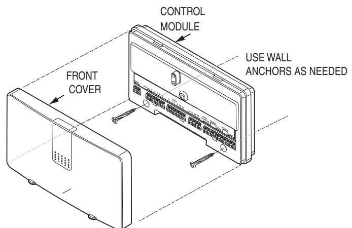
Figure 2. Control Module Locking Screws
