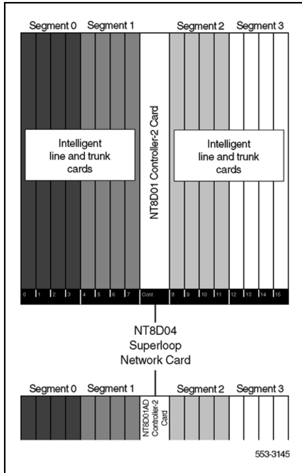
Figure 16 Eight segments per superloop
