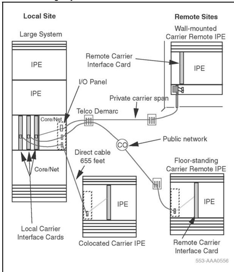
Figure 21 Meridian 1 Large Systemto Carrier Remote IPE links
