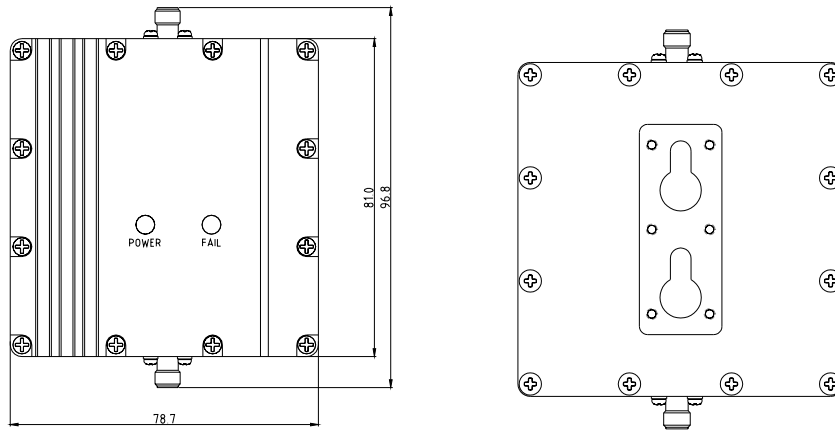
<Figure 5-1: USHR-800NI Front and Back views>
