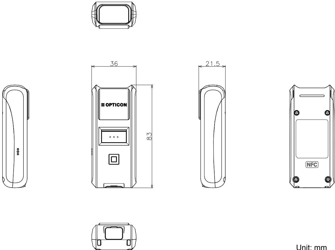
Figure 12: Mechanical Drawing
