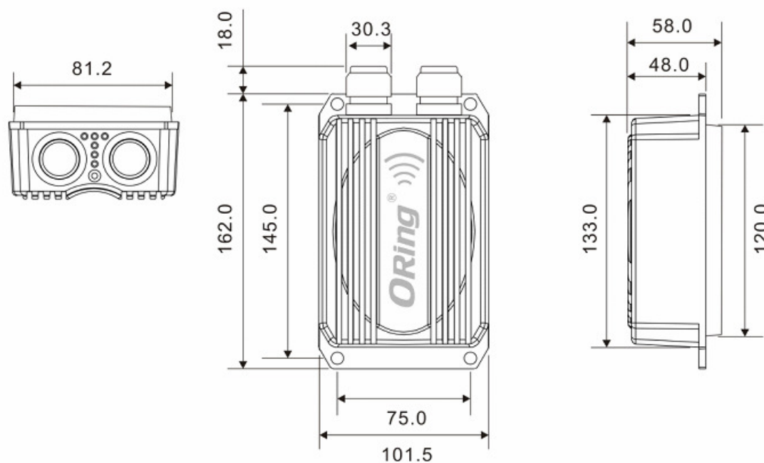
IAP-W420 Wall-mounting Measurements (Unit = mm)
