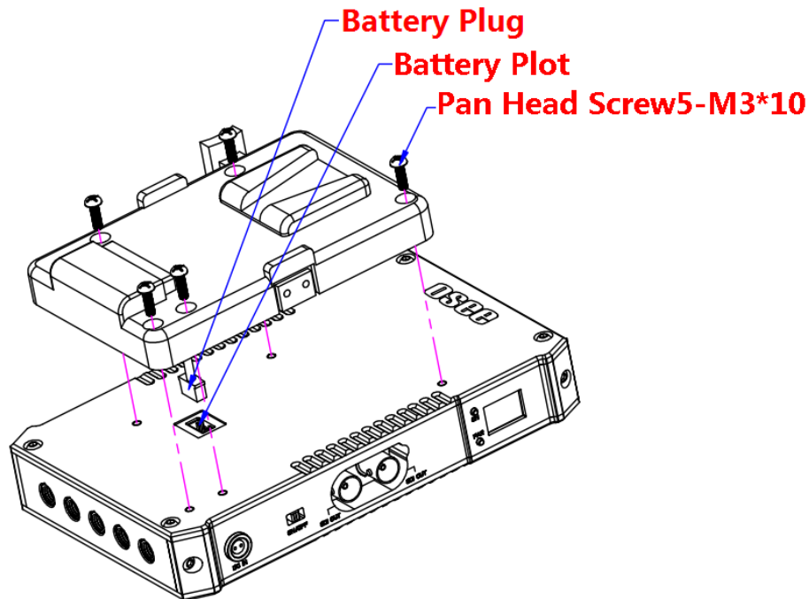
Figure 2-2 Battery Plate
