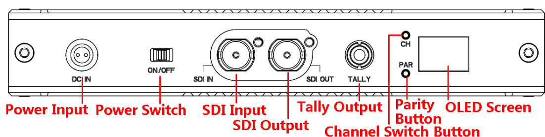
Figure 3.1-1 Left View of WVT-501 Transmitter
