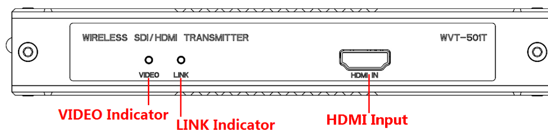
Figure 3.1-2 Right View of WVT-501 Transmitter
