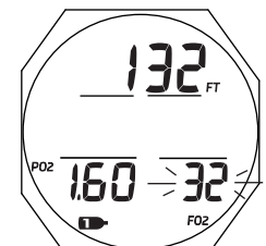
Fig. 37B - SET GAS 1 (FO2 for Nitrox)
