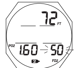
Fig. 38B - SET GAS 2 (FO2, then PO2 Alarm)
