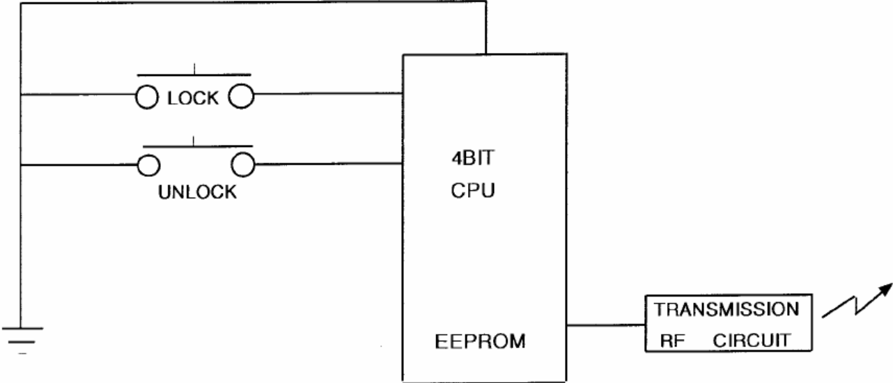
figure 3.1 block diagram of the transmitter
