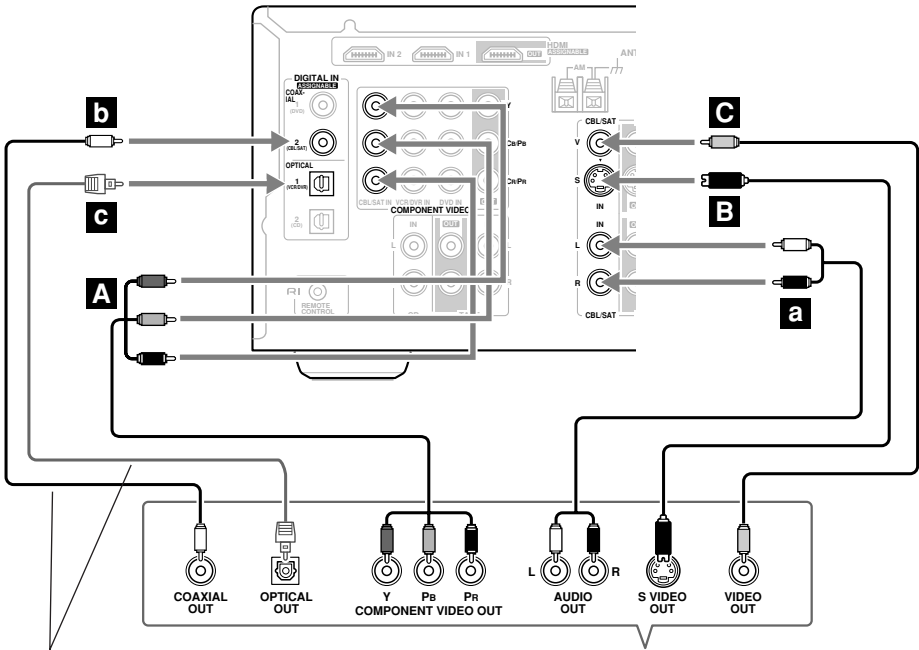
Satellite, cable, set-top box, etc.
