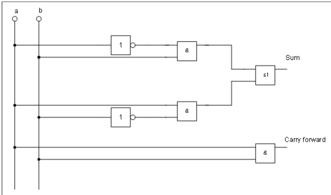
Figure 222: Half adder drawn using logic symbol building blocks
