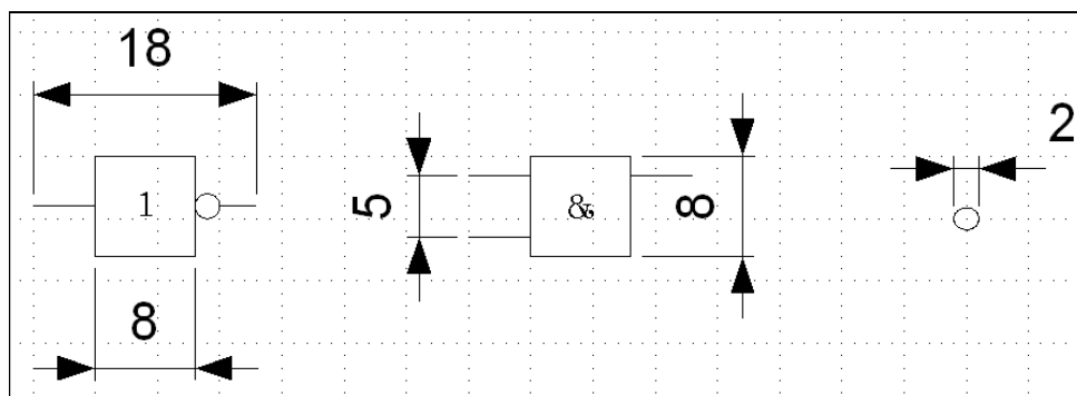
Figure 229: Dimensioned logic blocks
