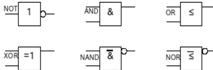
Figure 215: Logic Symbol library
