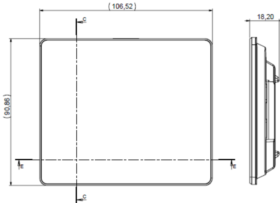
Figure 1: Dimensions
