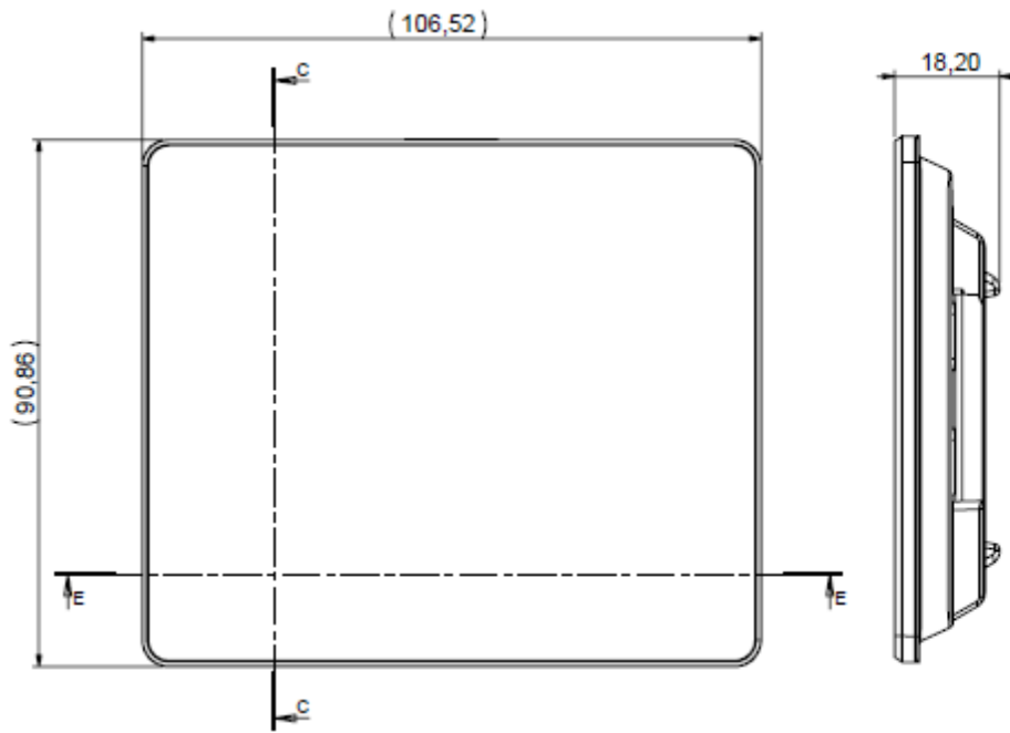
Figure 7: Mechanical drawing
