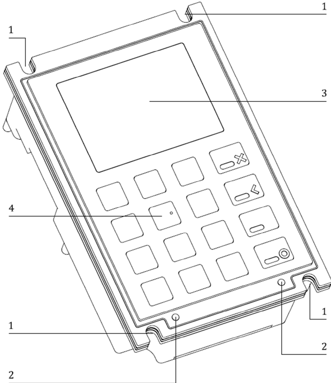
Figure 1: Front view
