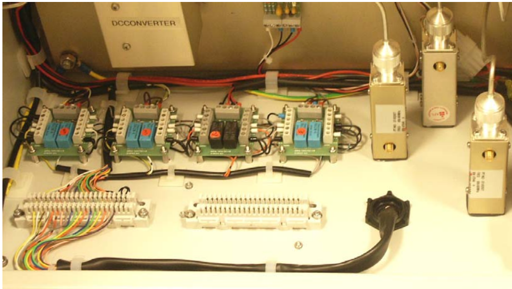
Inside Case Floor showing Alarm Krone Blocks & Relay PCB's
