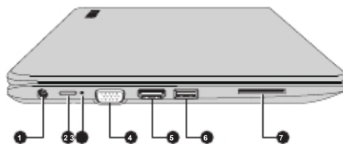
Figure 3-2 The left side of the computer (CL10-B/L10-B)
