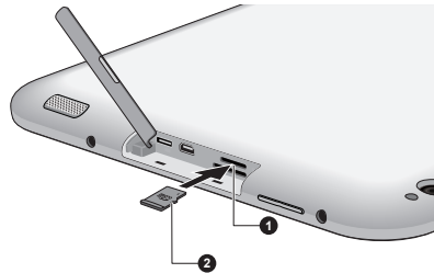
Figure 7-1 Inserting a memory media
