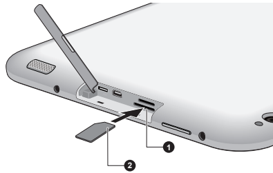
Figure 7-2 Inserting a SIM card
