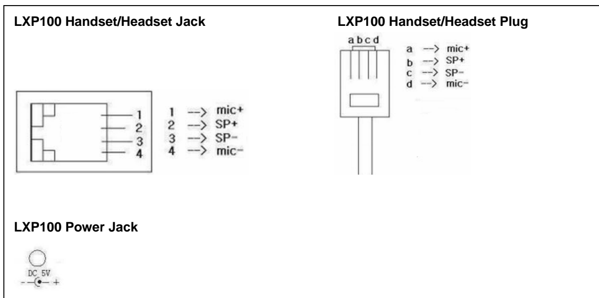
Figure 2: LXP100 Pin-out
