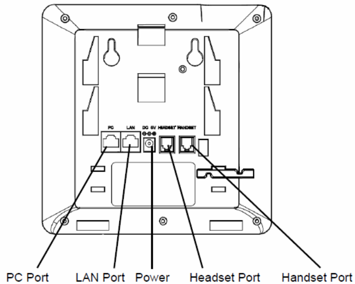
Figure 1: LXP100 Ports
