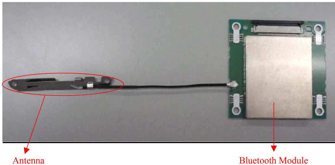
Fig 1. Front side of “C5ZZZ0000035 (C5ZZZ0000037)”
