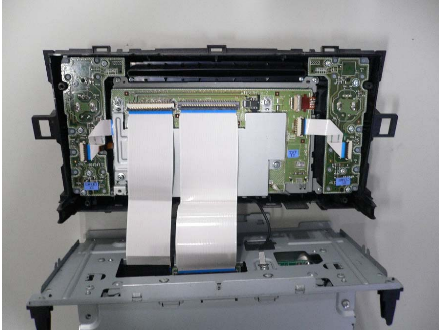
Fig 2. Top view of “YEAP01A727”, “YEAP01B897” be equipped for a Car Audio (example)
