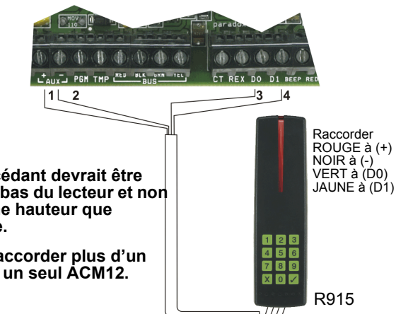
Figure 3 : Raccordement du R915
