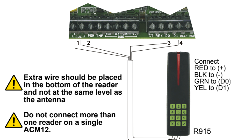
Figure 1: Connecting the R915 ACM12 (V4.0 or Higher)
