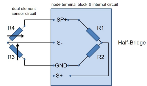
Figure 3 - Half-Bridge *
