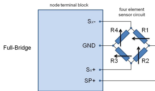
Figure 2 - Full-Bridge (Standard)
