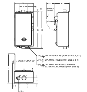
Figure 3 NEMA Type 4 Enclosure
