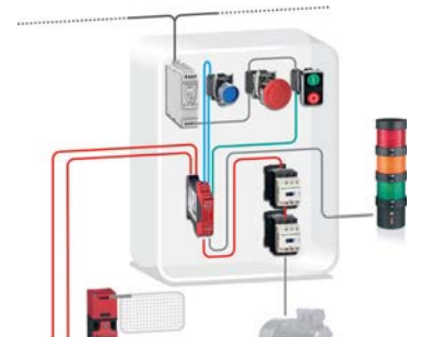
Safe stop 0 (PL e, SIL 3) High performance
