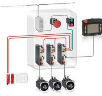
Safe stop 2 (PL e, SIL 3) Servo enhanced safety
