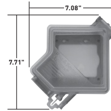
TWO GANG COVER
