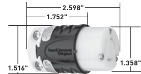
15A Connector
