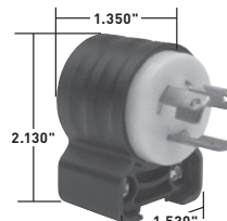
15 Amp Angle Plug
