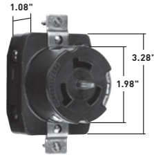
California Standard Receptacle
