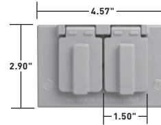
Horizontal 2 Self-Closing Lids
