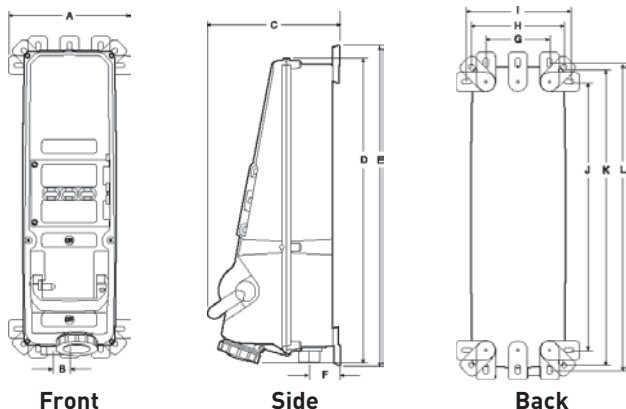
Hub shown at bottom of unit for reference only; may be field-installed for top or bottom entry. [See dimensions on Page I-5.]
