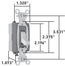
15 & 20 Amp Canadian 347VAC
