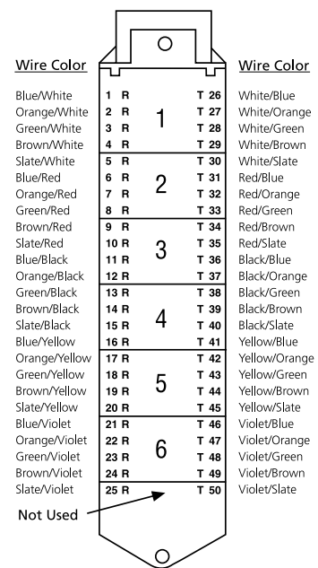
25-Pair Color Coding/ISDN Contact Assignment RJ-21X
