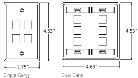
Single-Gang Dual-Gang Find wallplate Labeling Solutions on page A68.
