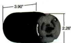
California Standard Connector
