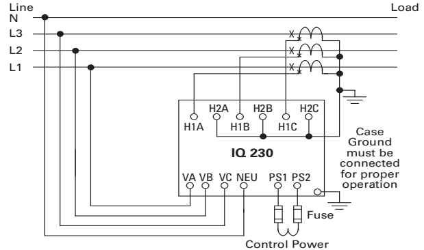
Three-Phase Four-Wire (up to 600 Volts) (Line Powered) Proper CT polarity is critical to the proper operation of the meter
