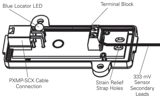
Open Interface Module (PXMP-IM333MV)
