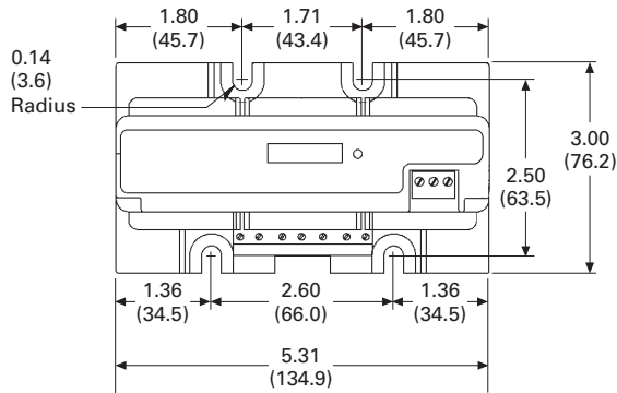
Universal with Internal CTs Energy Sentinels
