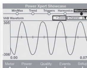
Waveform Viewer
