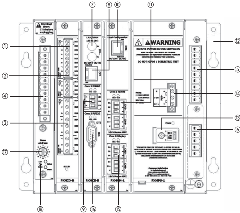
Power Xpert Meter 4000/6000/8000 Module Layout
