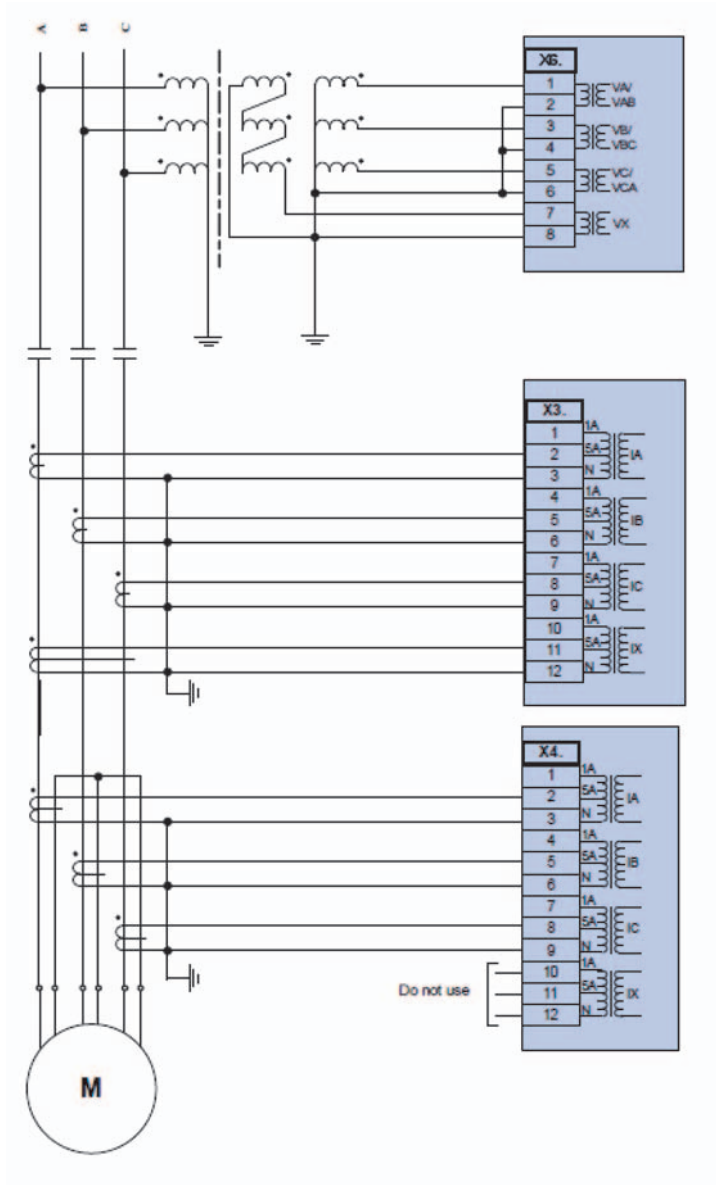
Typical AC Connections—Wye (or Delta) VTs, 5 A CTs, Ground Current Measured by 4th Zero Sequence CT, and 87 Motor Differential
