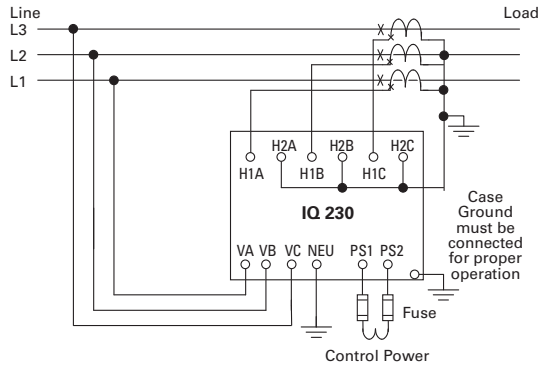
Three-Phase Three-Wire (up to 600 Volts) Proper CT polarity is critical to the proper operation of the meter
