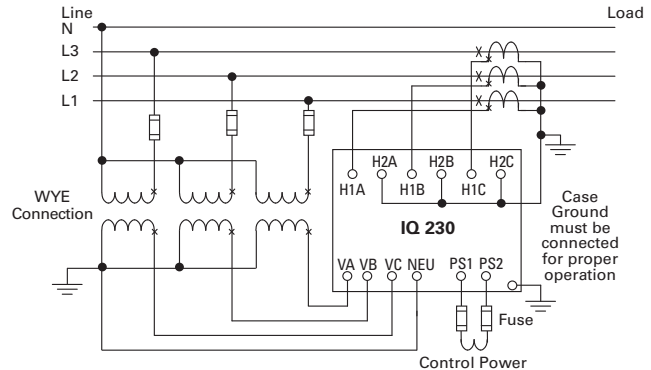
Three-Phase Four-Wire (above 600 Volts) Proper CT polarity is critical to the proper operation of the meter
