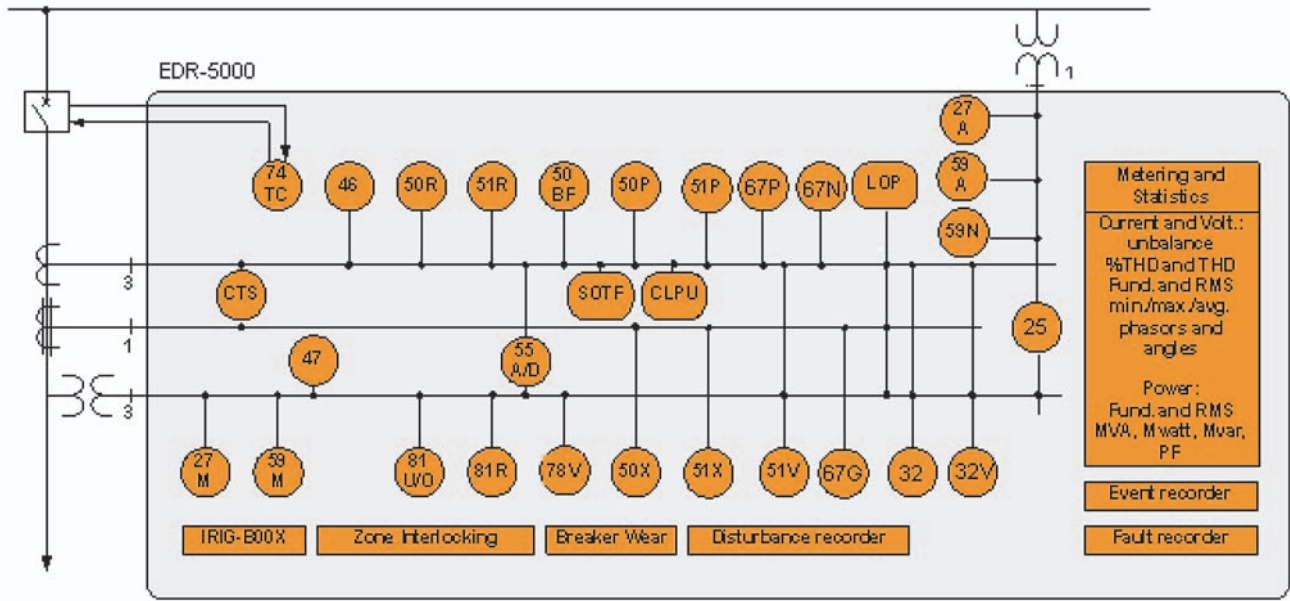
Typical One-Line Diagram
