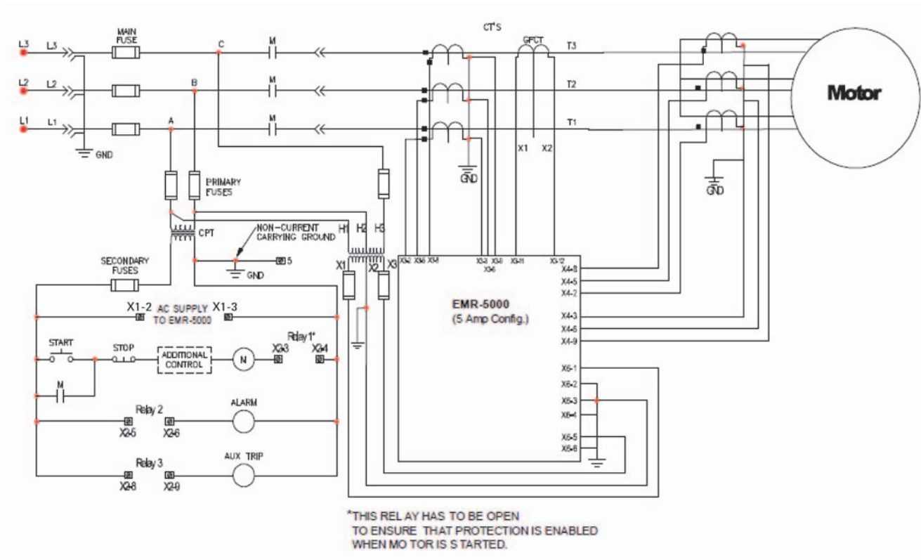
Typical Control Diagram
