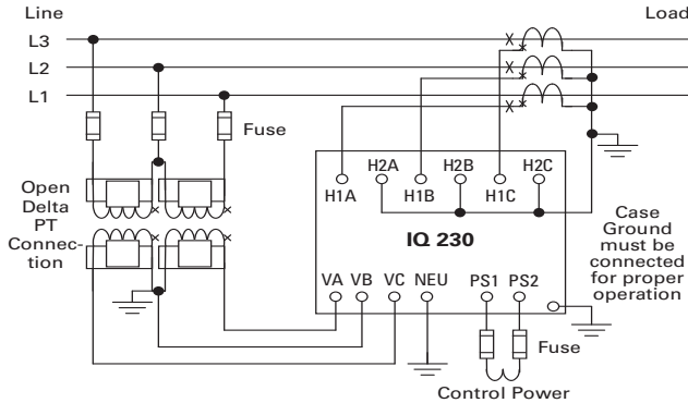
Three-Phase Three-Wire (above 600 Volts) Proper CT polarity is critical to the proper operation of the meter
