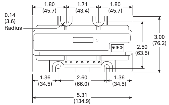
Universal with External CTs Energy Sentinels
