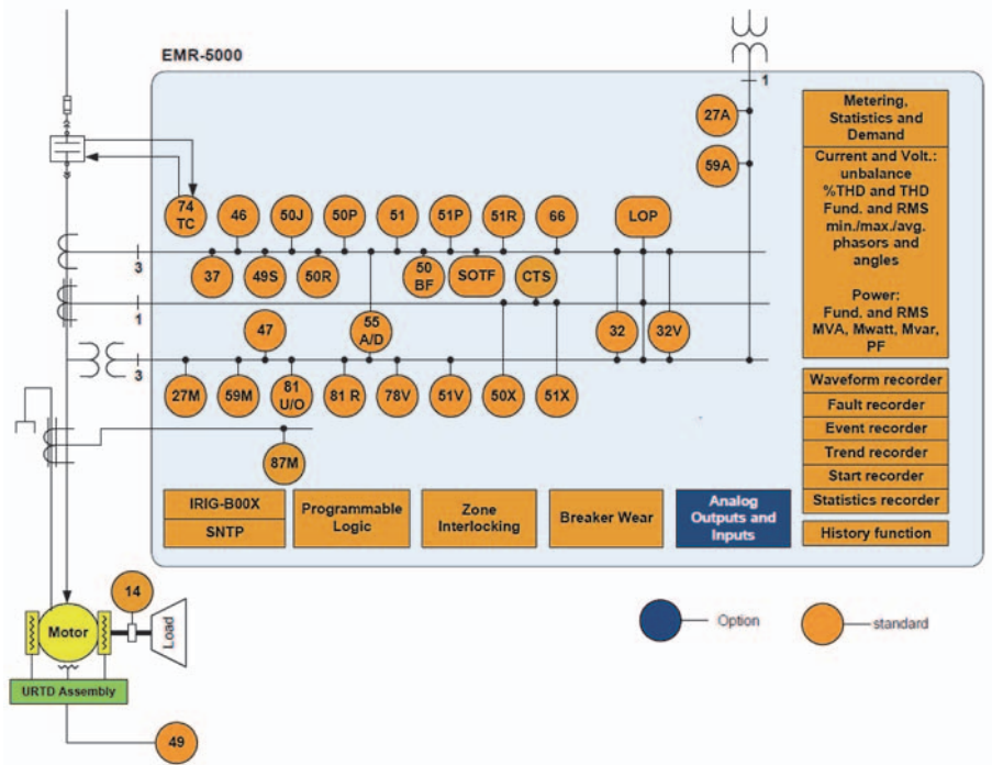
Typical Control Diagram
