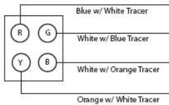
Datacom / Telephone
