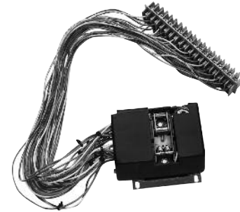
Auxiliary Switch with Pre-wired Secondary Terminals for Stationary Breaker
