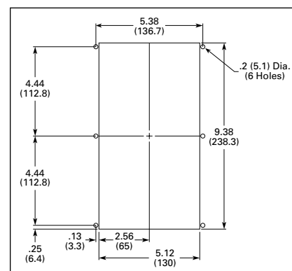
Figure A-64. Chassis Cutout Dimensions in Inches (mm)
