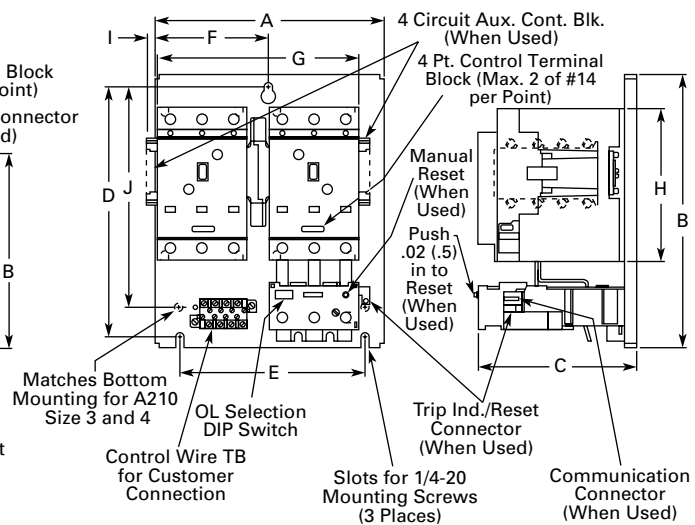
Figure 2 Sizes 3 and 4 Horizontal Reversing Contactor
