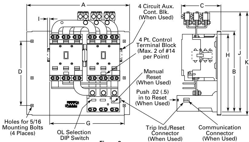
Figure 3 Sizes 5 and 6 Horizontal Reversing Contactor
