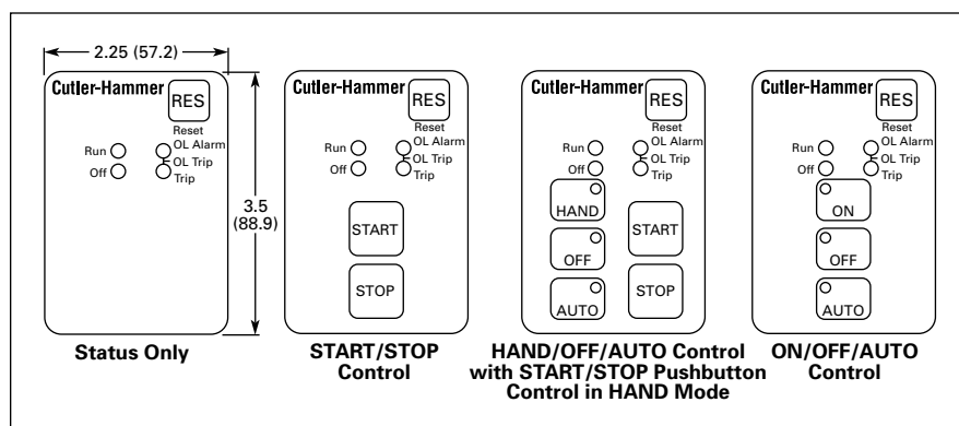
Figure A-54. Full Voltage and Reduced Voltage Control Modules
