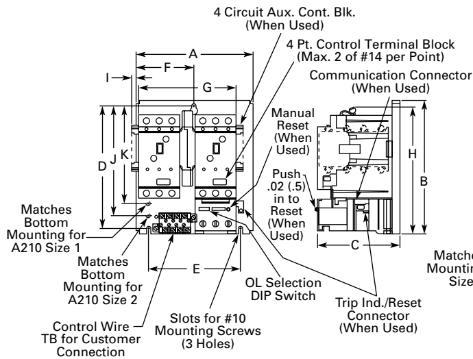
Figure 1 Sizes 1 and 2 Horizontal Reversing Contactor
