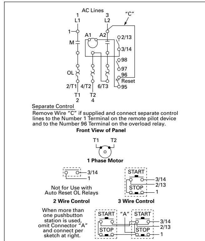
Figure A-16. Typical Wiring Diagrams — Single-Phase Applications (Factory Wired)
