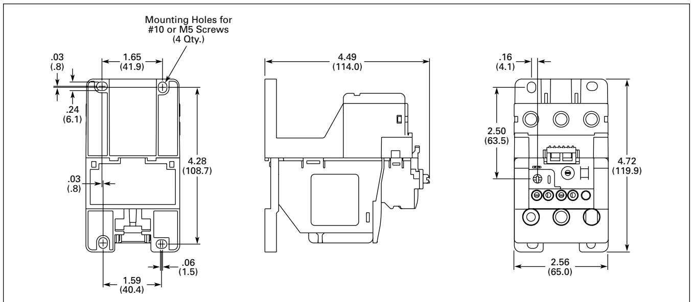
Figure A-39. 65 mm Stand-Alone C396 Electronic Overload Relay
