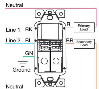
Sensor Wiring, Dual Circuit
