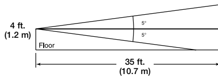
Dual Technology Sensor Field of View, Side
