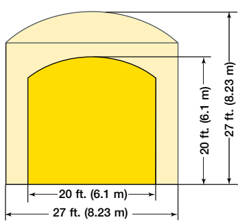
Ultrasonic Sensor Field of View, Top
