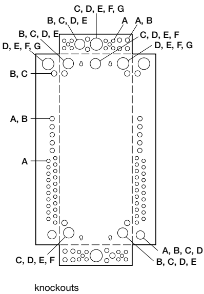
36M Knockouts
