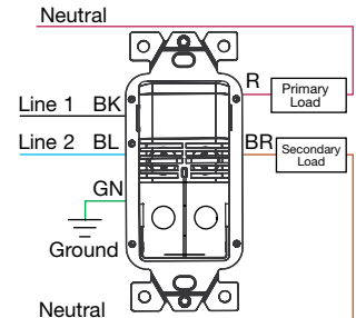
Sensor Wiring, Dual Circuit
