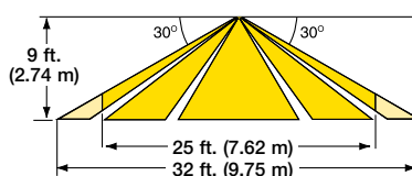
Side view of sensor field of view
