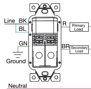
Sensor Wiring, Bi-level
