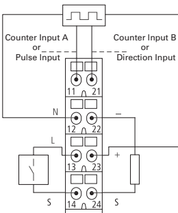
XNE-2CNT-2PWM
