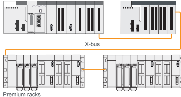
Modicon M580 Modicon X80 expansion rack
